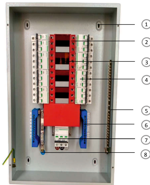
TPN MCB BOARD ( MD Series )
